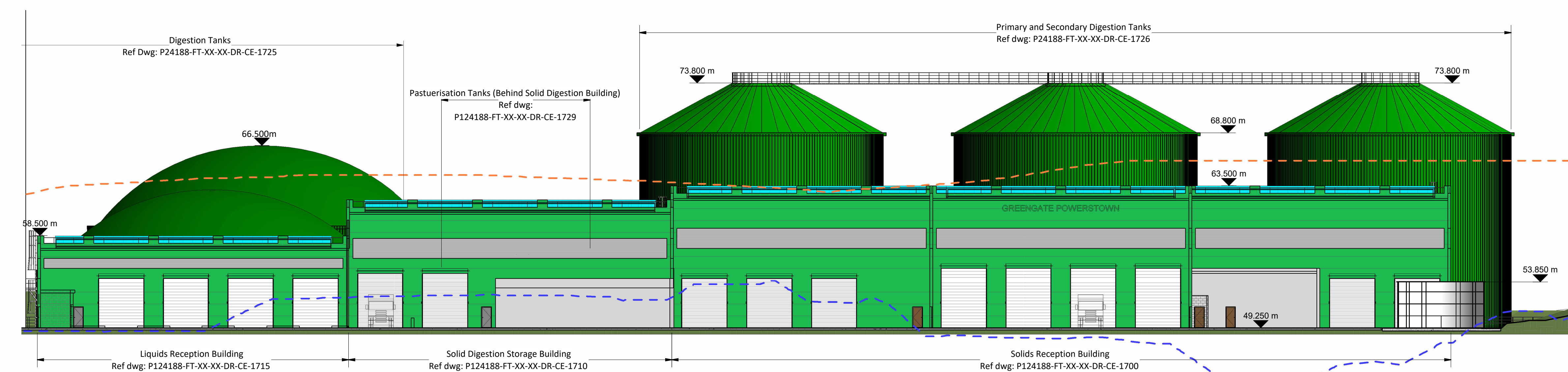
SITE CROSS SECTION - DETAIL 2 Scale 1 : 250
